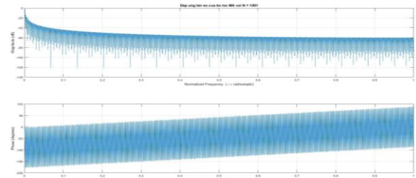
Figure 7. Frequency response of the MA filter with N = 1001 .
