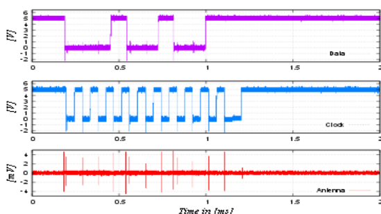
Fig.5. Data signal, Clock signal and radiated signal of PS/2 keyboard when key E is pressed [8]
