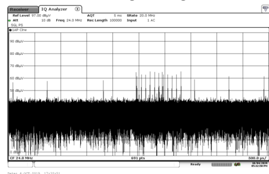
Fig.9. Radiated signal of key A is captured in near field
