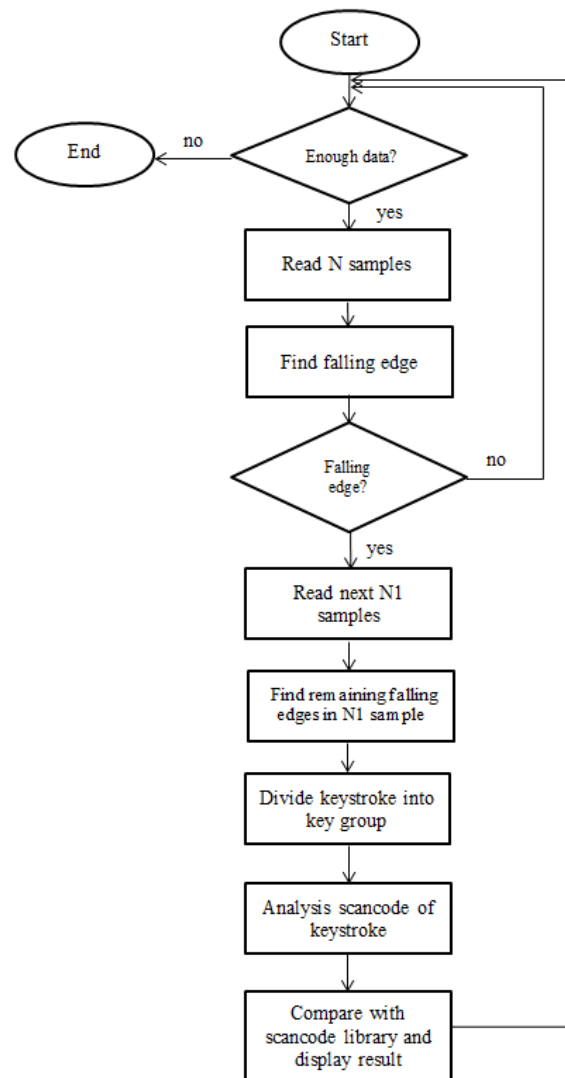
Fig.8. Algorithm flowchart of analyzing radiated signal process
