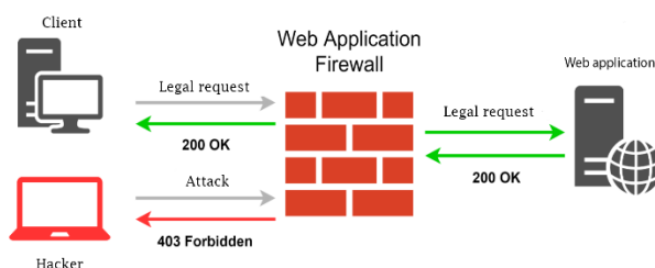
Fig.1. WAF in Web Application Security System
