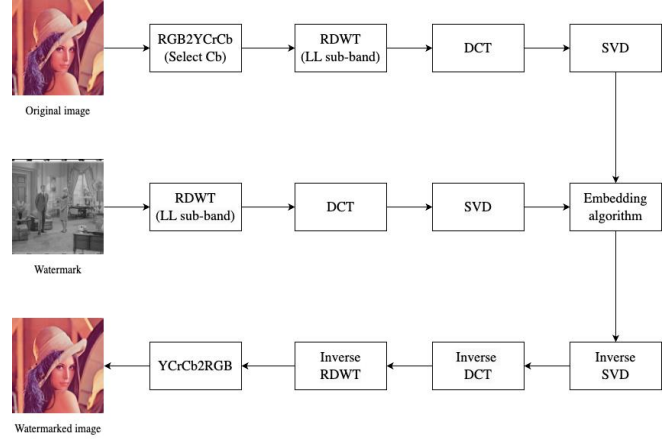
Figure 1. The watermark embedding process
