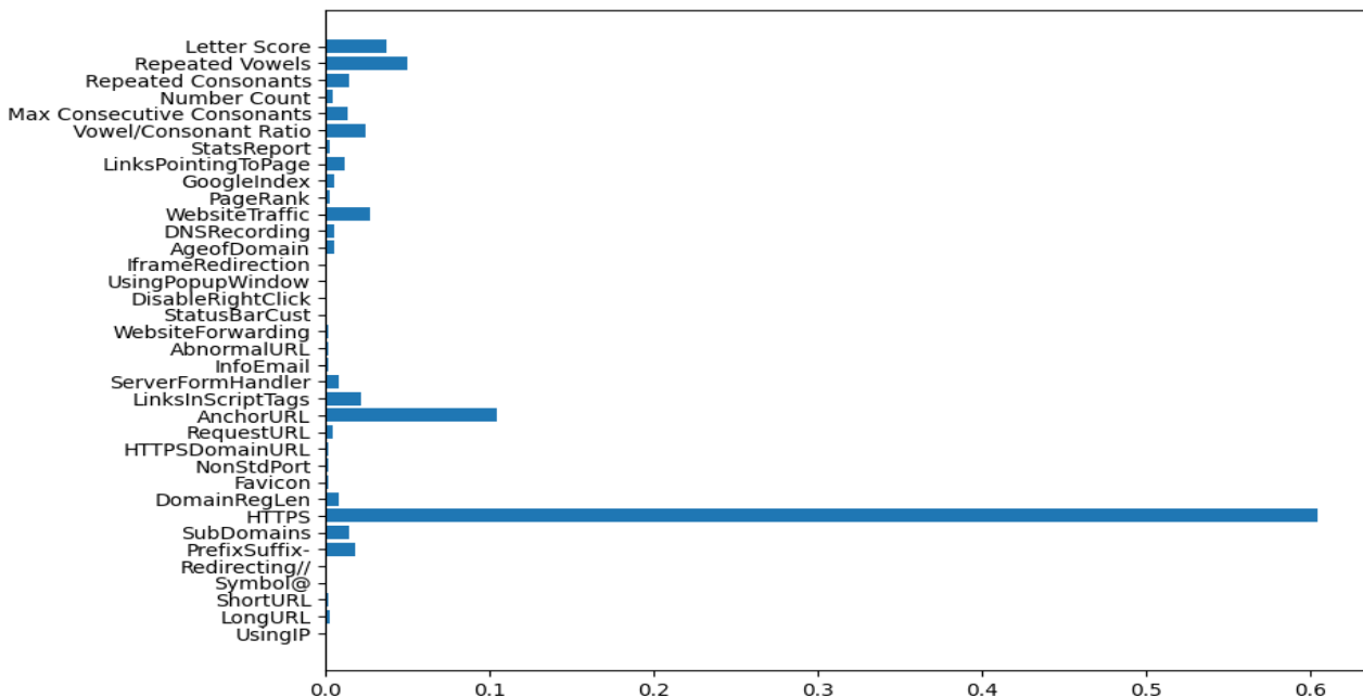
Figure 2. Features importance
